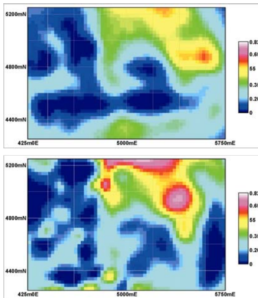
Figure 5. Chargeability model plan sections, 420m RL (80m below lowest point on survey grid) - 2D3D (top) and 3D3D (bottom). Note the significant improvement in resolution of structures for 3D3D.
