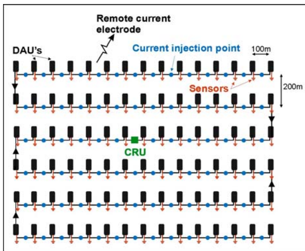
Figure 2. Layout for acquiring 3D IP data at Scotch Prospect, Copper Hill. Data were collected over the entire array for each current injection. DAU's send data back to the CRU via the network at the end of each event. Data path is indicated by black arrows.
