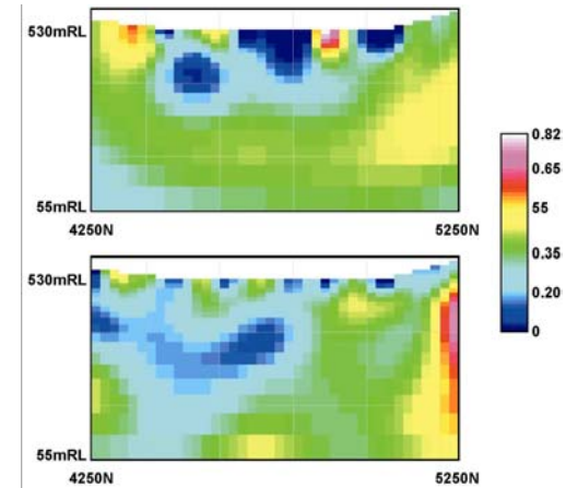
Figure 7. Chargeability model sections for 2D3D (top) and 3D3D (bottom) – 5000E. Note the poor definition of structures in the top section.
