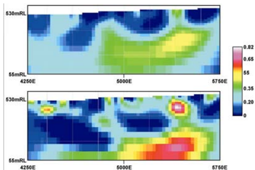
Figure 6. Chargeability model sections for 2D3D (top) and 3D3D (bottom) – 4725N. Note the improvement in resolution for the 3D3D section.
